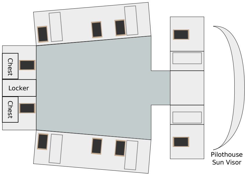
Aft Deckhouse
